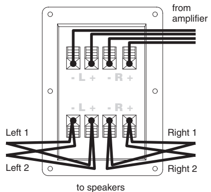
Figure 19: Direct wiring plan
