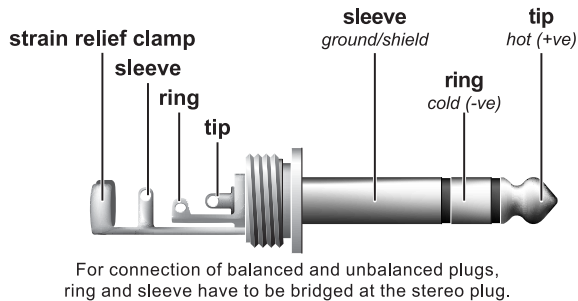
Fig. 8.3: 1/4" TRS connector
