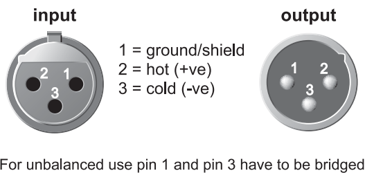
Fig. 8.1: XLR connections
