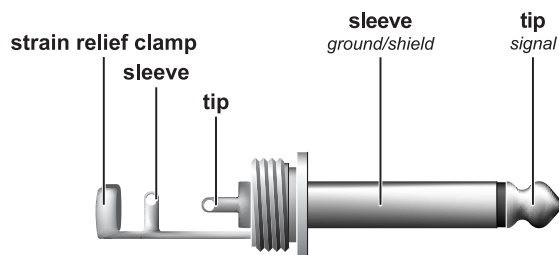
Fig. 8.2: 1/4" TS connector
