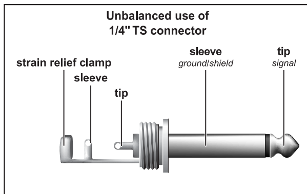
Fig. 8.2: 1/4" mono plug
