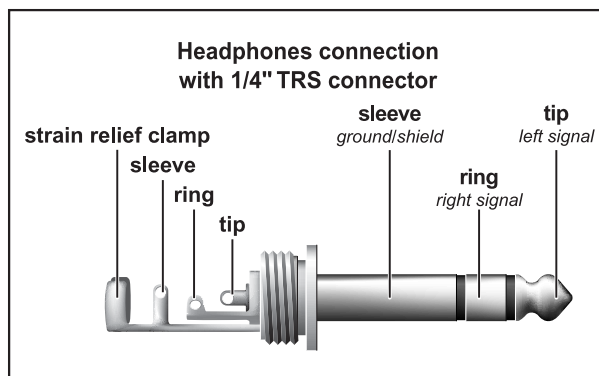
Fig. 8.4: Stereo headphones 1/4" plug
