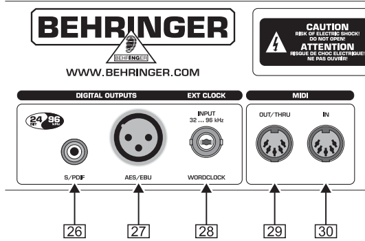
Fig. 2.6: V-AMP PRO rear panel (section 2)
