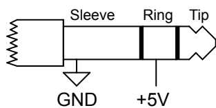
Connector Wiring Diagram
