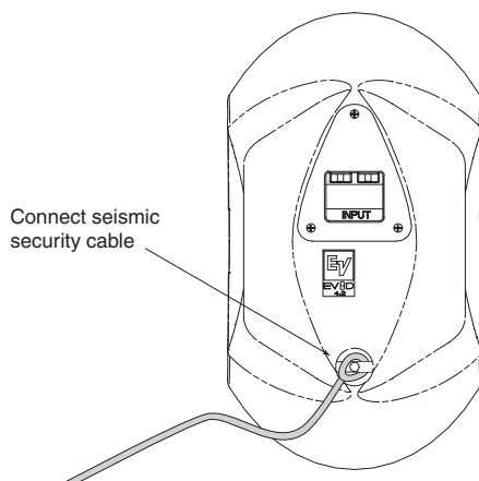
Figure 12: Secure seismic security cable
