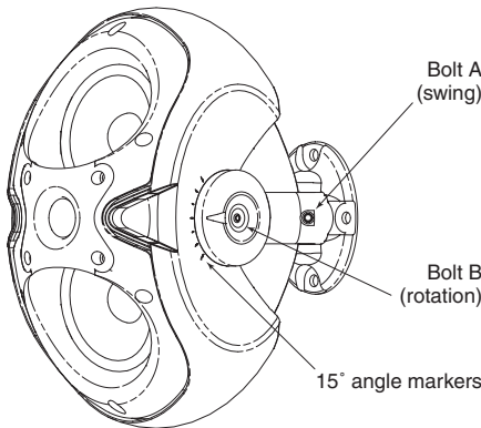
Figure 10: Tighten socket-head bolts
