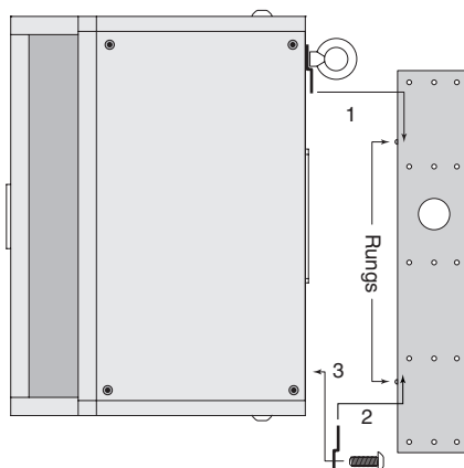
Figure 21: Corner mounting
