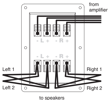
Figure 19: Direct wiring plan
