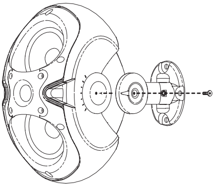
Figure 9: Attach SAM™
