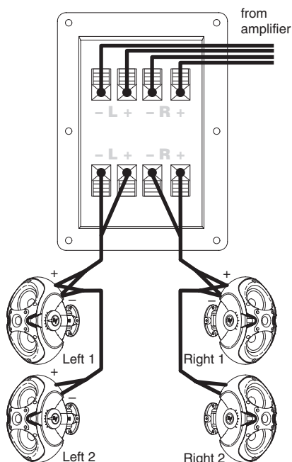
Figure 20: Daisy-chain wiring plan
