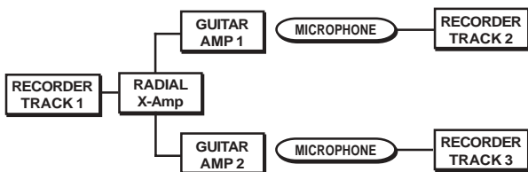
Example using two guitar amps recorded to separate tracks
