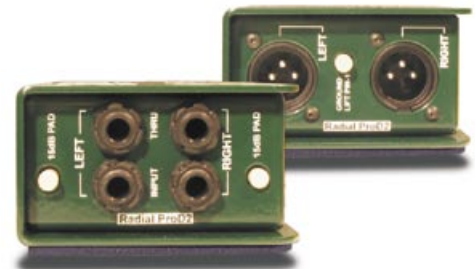
The ProD2 is two independant direct boxes in one package: two inputs, thru-puts, pads, transformers, outputs.
