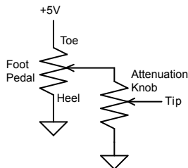
Pedal Schematic
