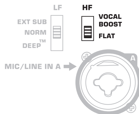
KW122, KW152, KW153 High-frequency EQ Switch
