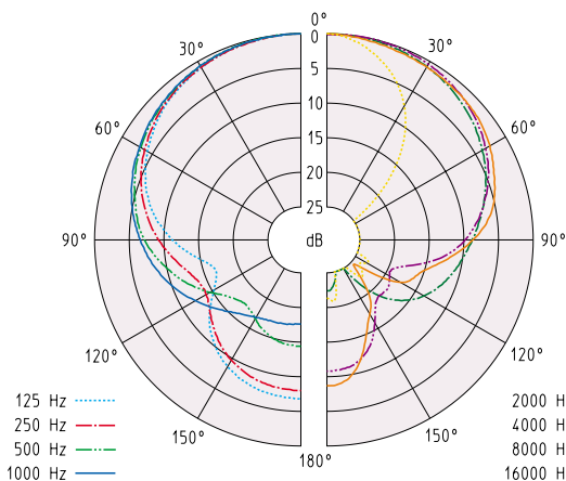
Polar Pattern
