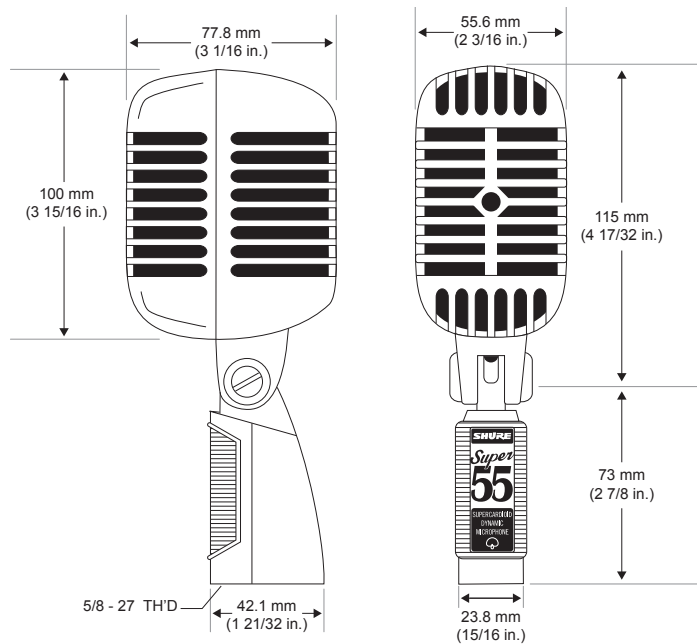
OVERALL DIMENSIONS
