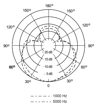
TYPICAL POLAR PATTERNS
